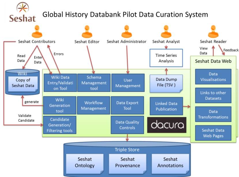
Fig. 4. Seshat Ontology Deployment in Data Curation System
